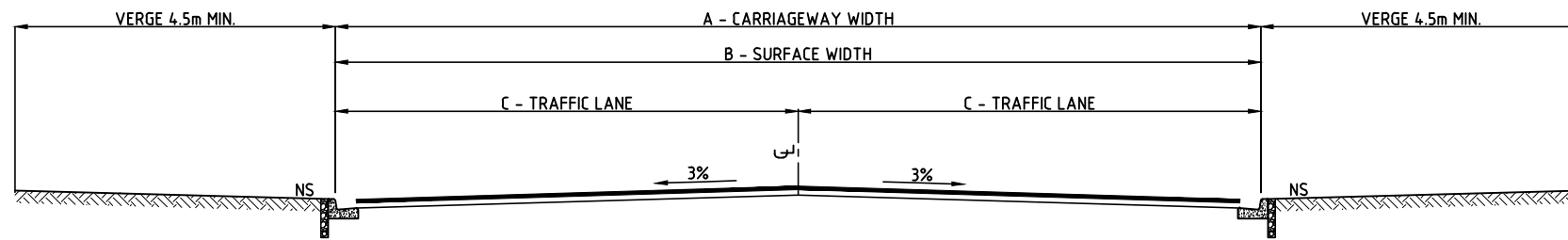
CROSS SECTION TYPE 1 URBAN INDUSTRIAL WITH SEAL SURFACE & KERB & CHANNEL DRAINAGE
