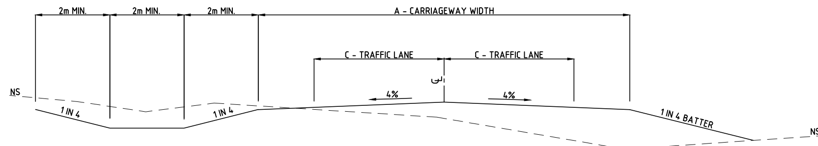
CROSS SECTION TYPE 3 RURAL LOTS GREATER THAN 20ha & PASTORAL PROPERTIES WITH GRAVEL ROAD TYPICAL CROSS SECTION
