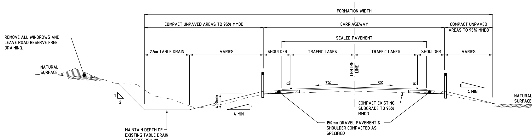
TYPICAL CROSS SECTION SEALED ROADS REFER TO TABLE FOR TRAFFIC LANE, SHOULDER AND CARRIAGEWAY WIDTHS.
