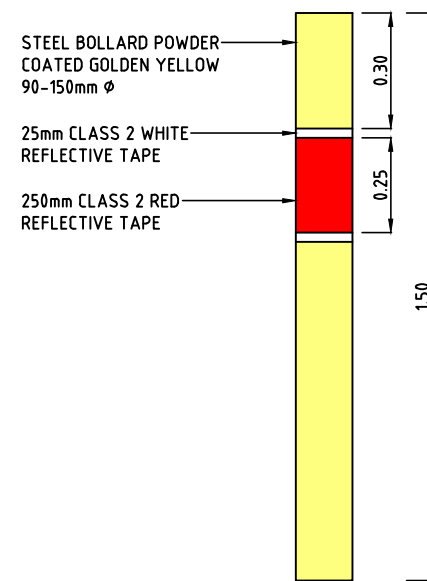
TYPICAL BOLLARD
