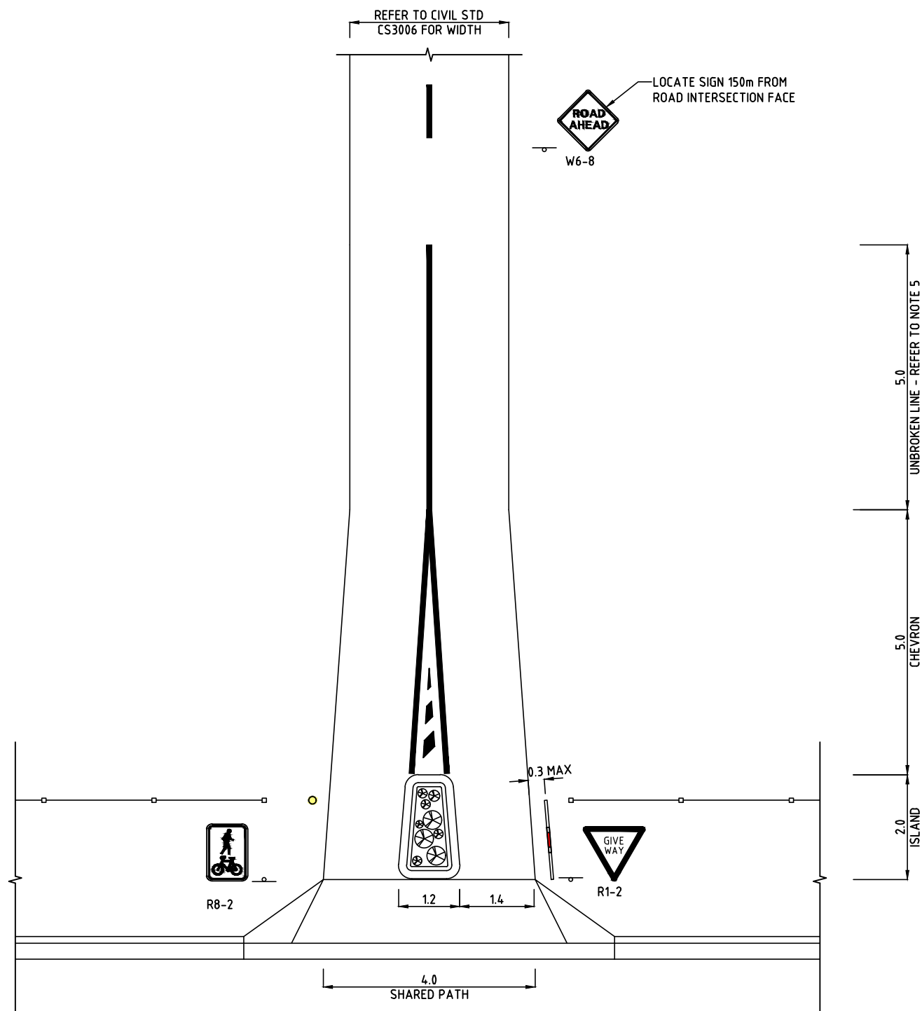
PLAN VIEW
