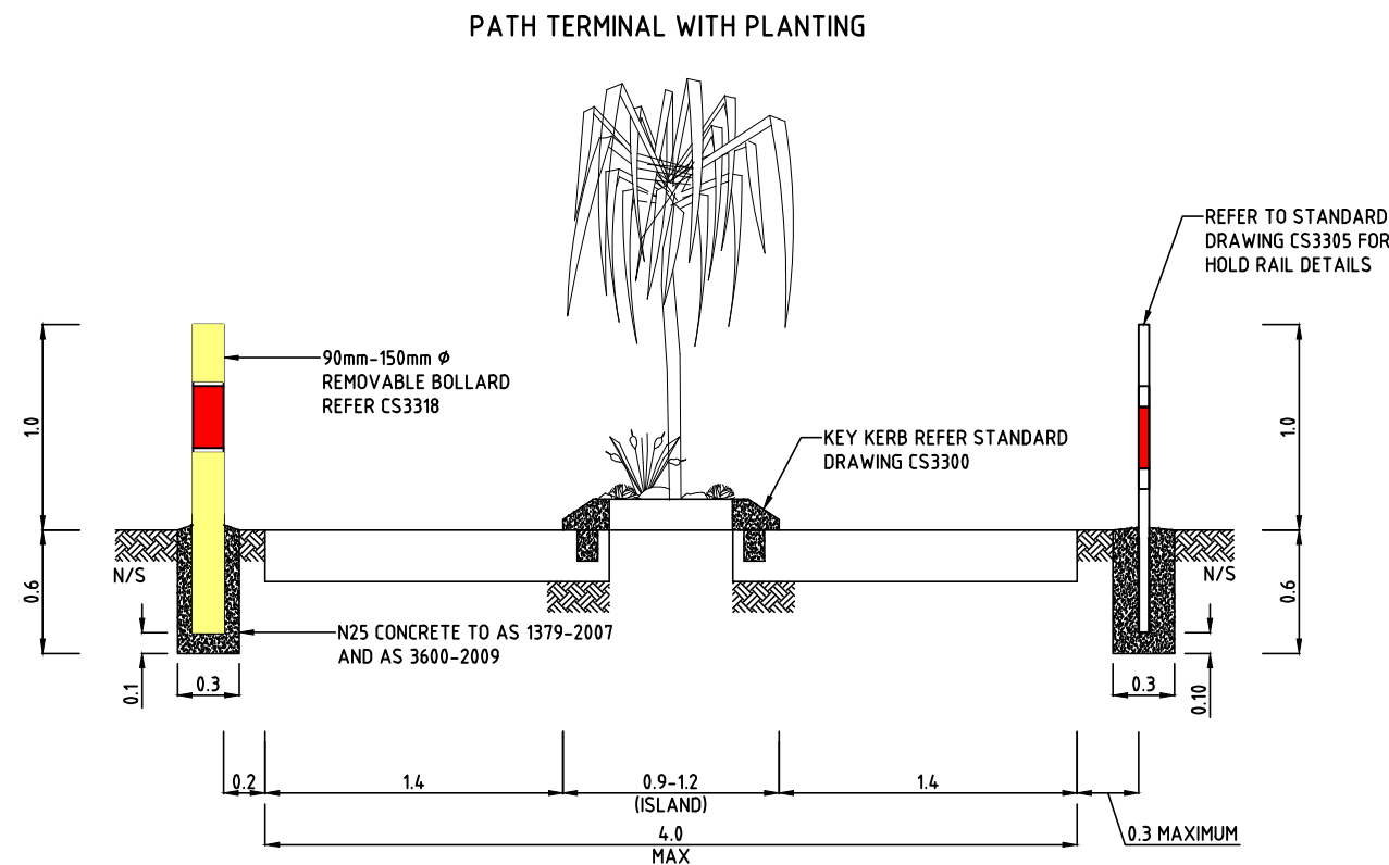
TYPICAL SECTION
