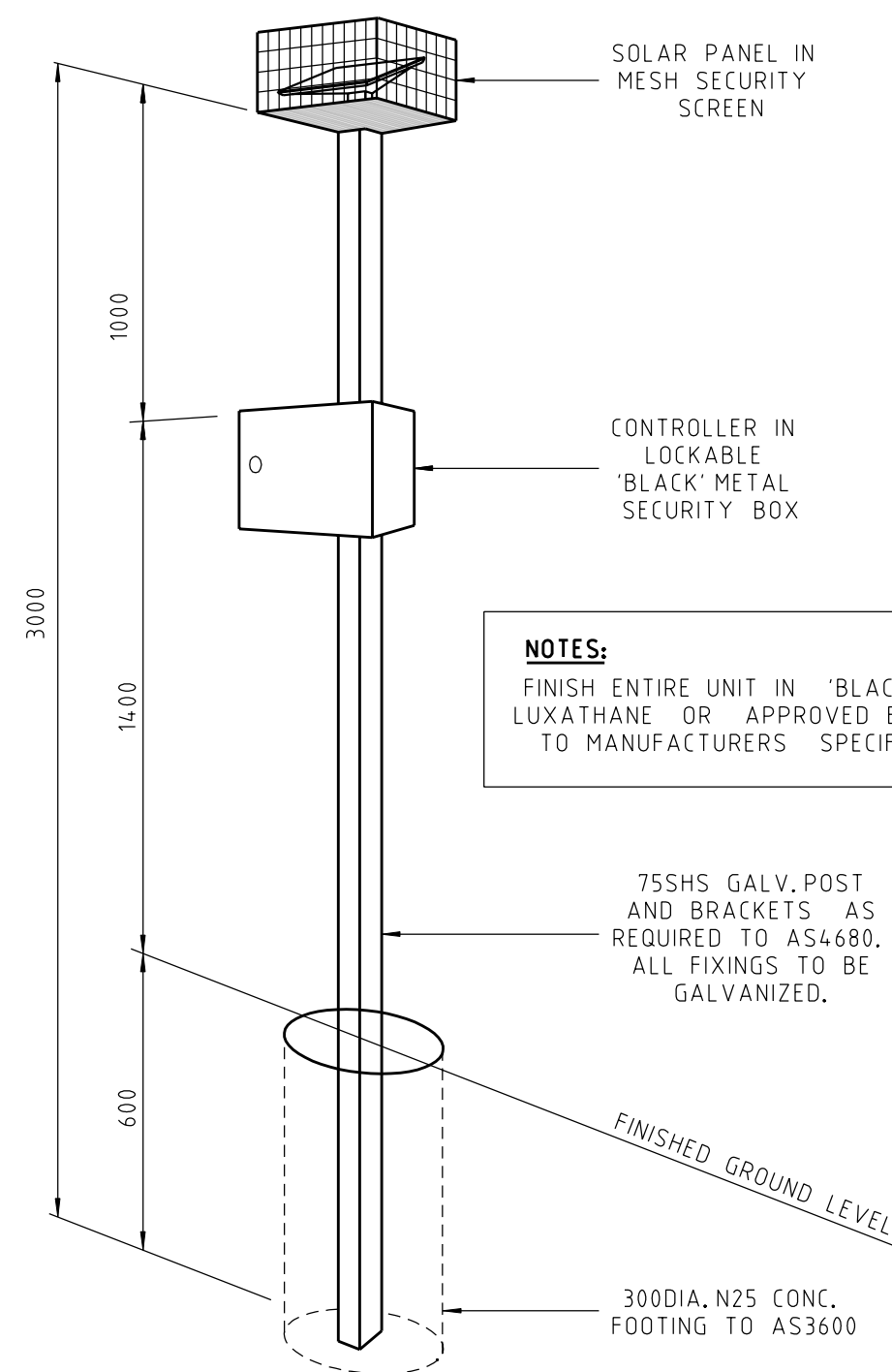
TYPICAL SOLAR CONTROLLER
