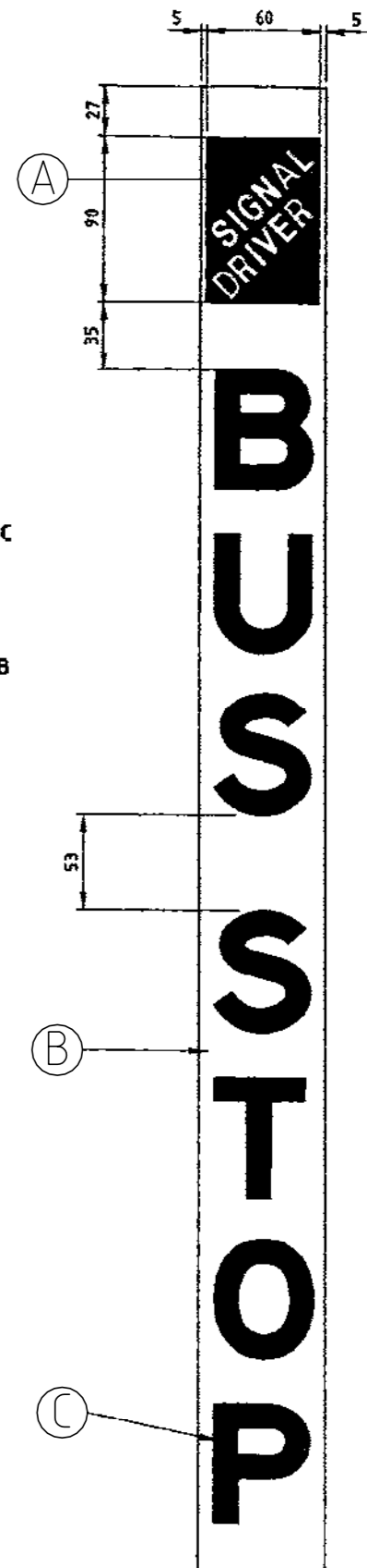
BUS STOP STICKER DETAIL NTS
